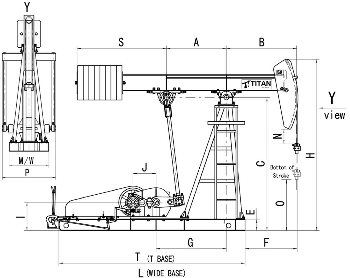
Titan Beam Balance Pumping Unit Dimensions (Inches)
